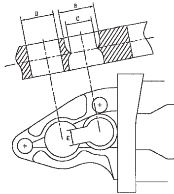
S/S THRUBAR SHROUD SEAT DETAILS
